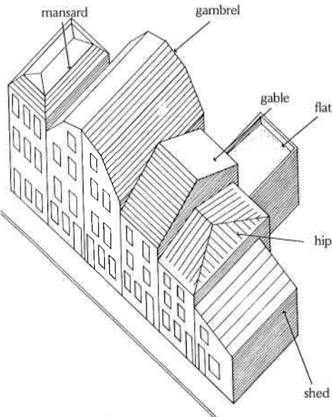
Roof shapes.
