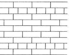
Common bond
